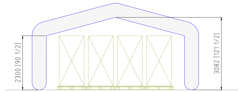
FRONT SECTION
